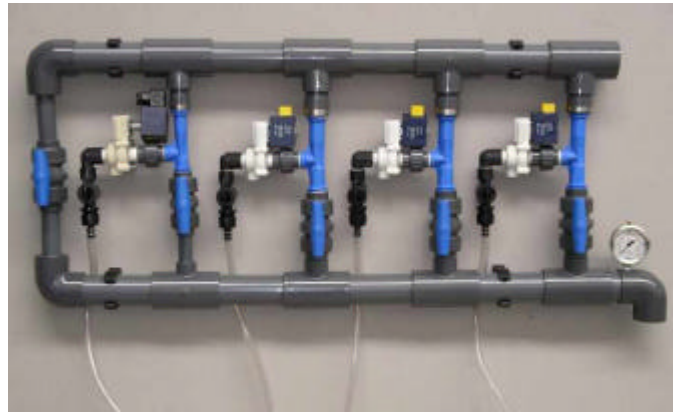
Pre-assembled venturi manifold for in-line injection
